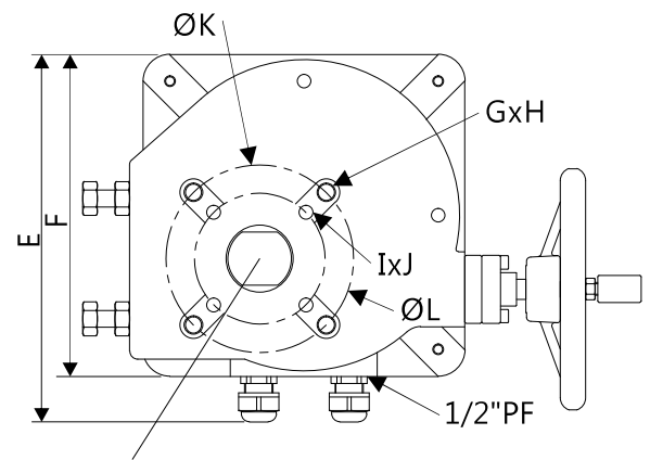
Shaft Type 1
