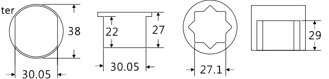
Shaft Type 1
